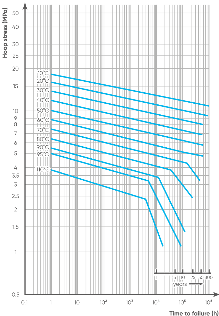
Minimum required hydrostatic strength curves for PP-R.
