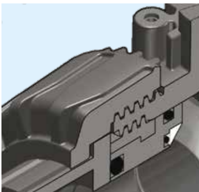
The ball seat carrier is manufactured in two pieces, one external threaded piece for assembly and one internal piece where the seals are located.
