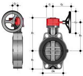
FEOV/RM Gearbox operated Butterfly valve
